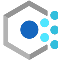
Azure Policy
